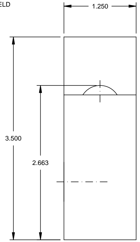
SECTION AT CABLE ENTRY
